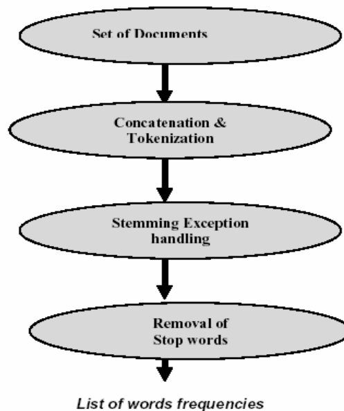
Figure 7. steps in pre-processing
