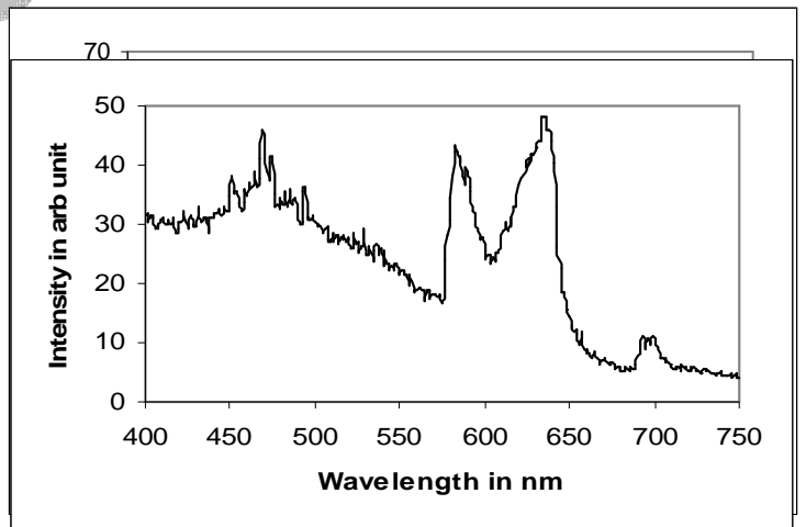
Figure 2 represents Emission spectra of BaMgAl 10 O 17 : Sm (2 %) with Excit. at 254 nm.
